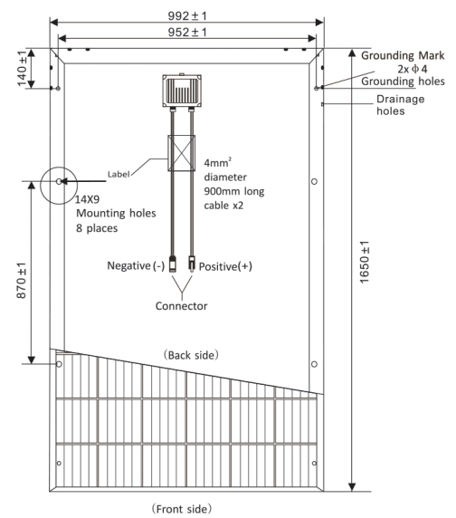
Dimension of PV Modules Unit: mm
